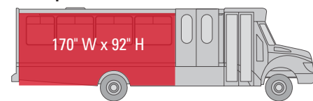
Champion Queen - curb side
