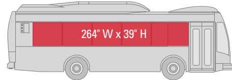
Gillig King Window - curb side
